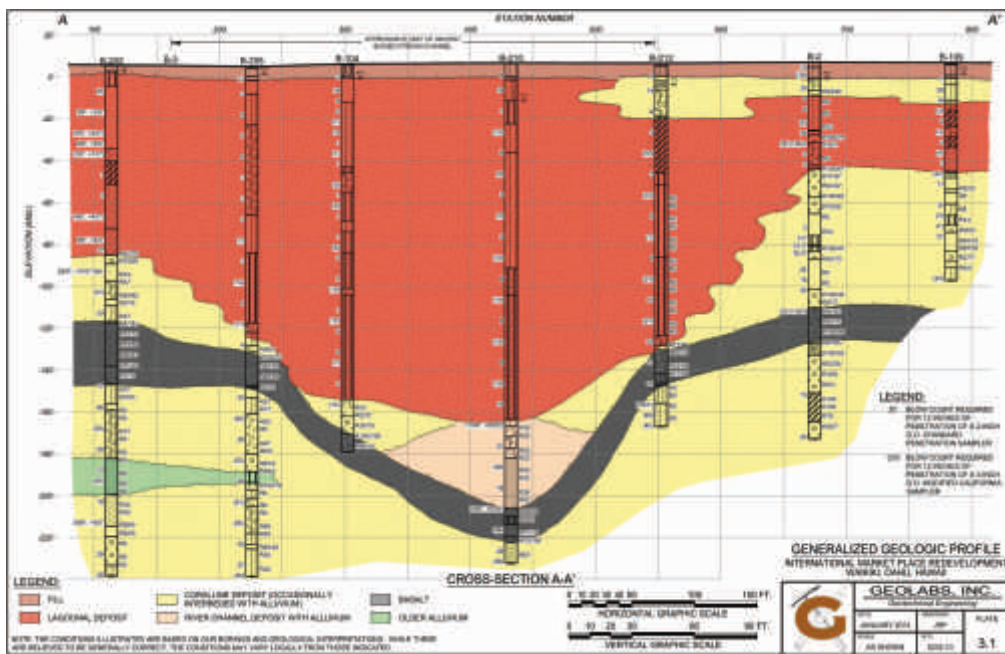
Generalized north-south geologic profile of the site
